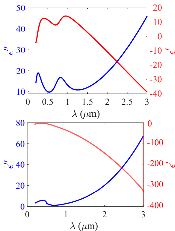
Fig. 1 Dispersion of the dielectric function of (a) titanium carbide 1 and (b) gold as a function of wavelength.
