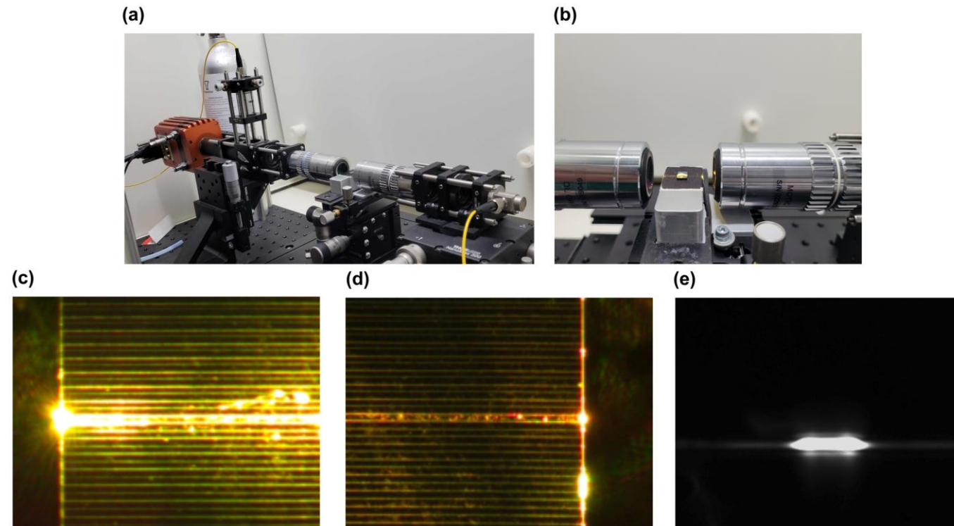
Figure 12: Photographs of an experimental setup for waveguide coupling and observation of output mode.
