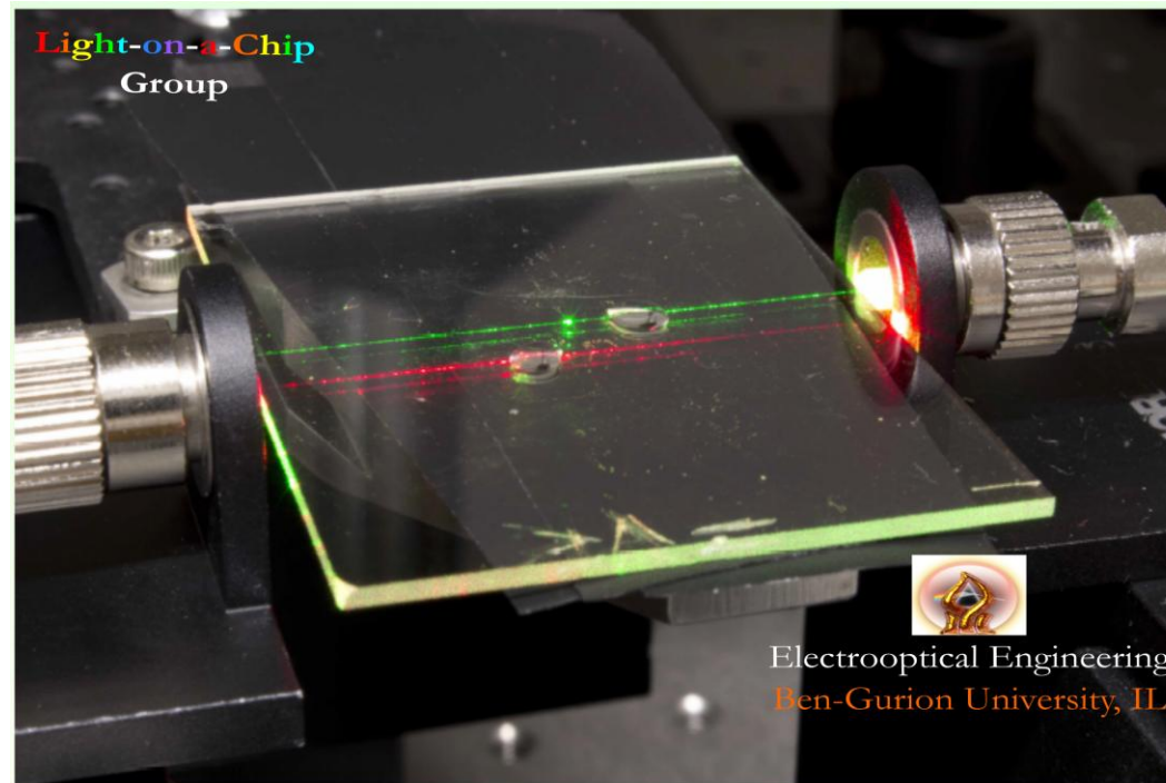
Figure 14: Butt-coupling to a channel waveguide.
