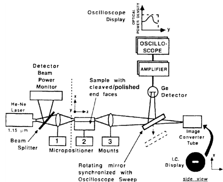
Figure 13: Diagram of an experimental setup that can be used to measure optical mode shapes [2].
