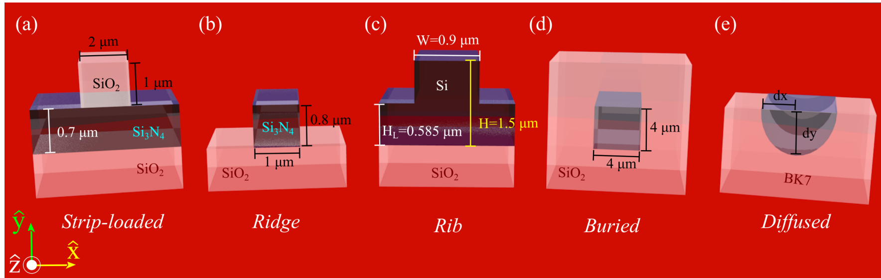
Figure 9: Common laterally confined passive waveguide structures: (a) a strip-loaded waveguide made of nitride on a silica substrate covered by silica, (b) a ridge waveguide made of nitride on a silica substrate, (c) a rib waveguide made of silicon on a silica substrate, (d) a waveguide buried in silica glass, and (e) a diffused waveguide in borosilicate glass [1].
