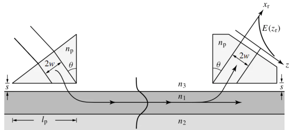
Figure 15: coupling using prism couplers [from Fosco.]
