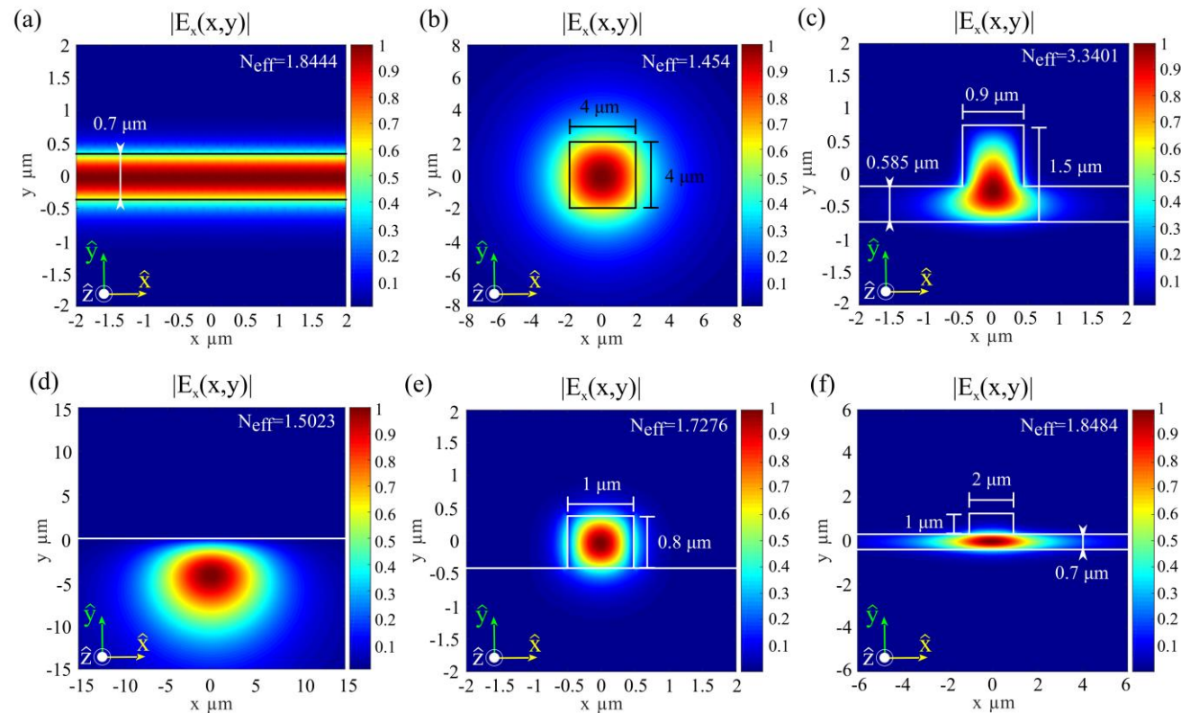
Figure 10: Quasi-TE polarization. Colormaps of |E_x(x,y)| , normalized to the maximum amplitude in single-mode waveguides: (a) slab, (b) buried, (c) rib, (d) diffused, (e) ridge, and (f) strip-loaded [1].
