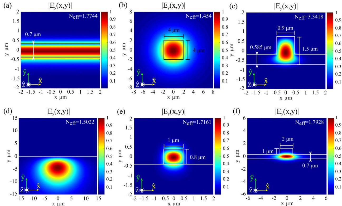
Figure 11: Quasi-TM polarization. Colormaps of |E_y(x,y)| , normalized to the maximum amplitude in single-mode waveguides: (a) slab, (b) buried, (c) rib, (d) diffused, (e) ridge, and (f) strip-loaded from [1].
